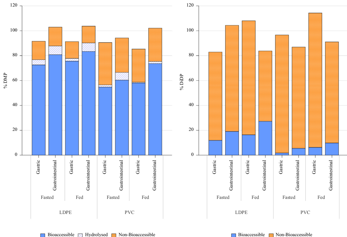
Fig. 2. Stacked barplot of hydrolyzed amount, bioaccessible and non-bioaccessible fractions for DMP (left) and DiDP (right) based on microplastic type, PBET model and body fluids.
